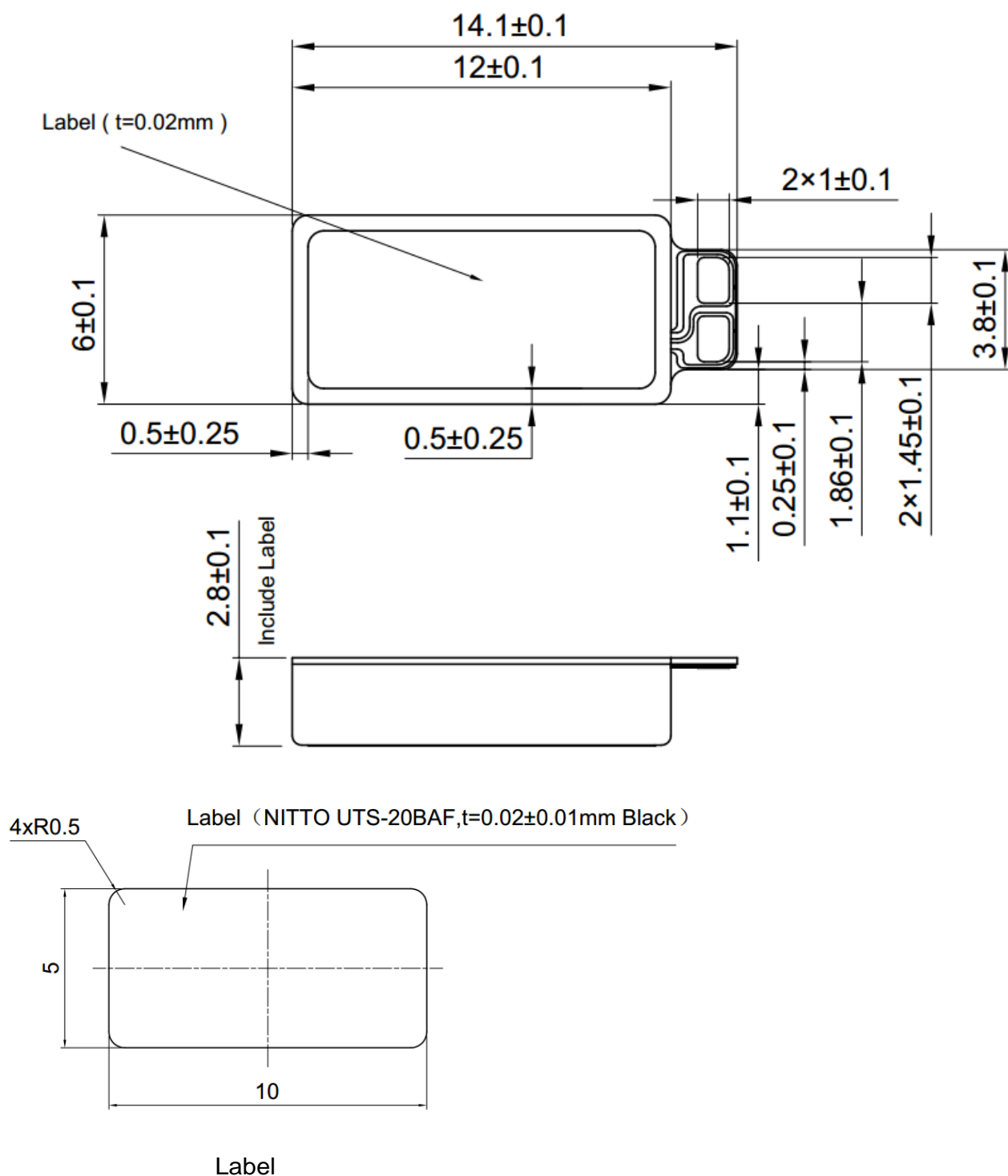
Fig 4. mechanical layout
