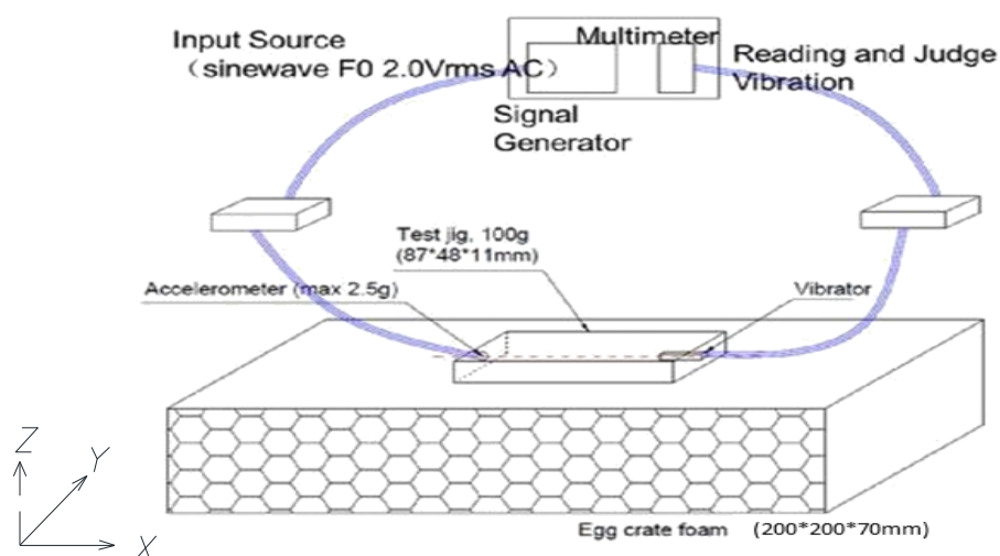
Fig 2. test method
